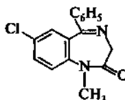
дiazepam
